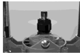
Fig. 15 Conical adapter M12 x 1 mm, nut tightened
